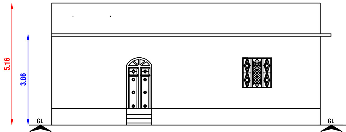
FRONT ELEVATION
