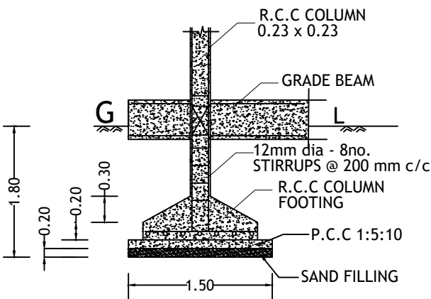
COLUMN - FOUNDATION DETAILS
