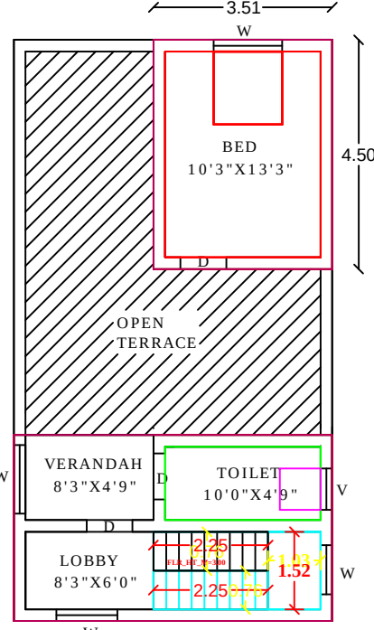
PRO.SECOND FLOOR PLAN
