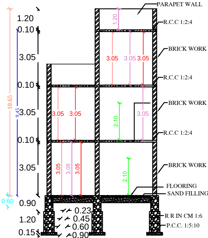
SECTION AB
