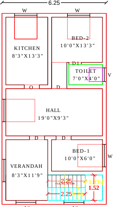
EXG.FIRST FLOOR PLAN
