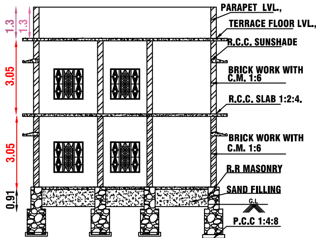
SECTION ON A-A & A'-A'
