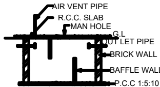
SECTION ON SEP. TANK
