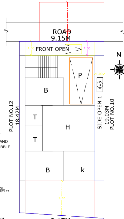
RAIN WATER HARVESTING
