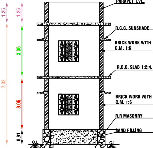
SECTION ON A-A & A'-A'
