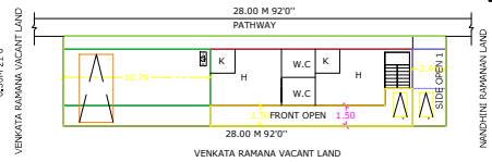
SITE PLAN SCALE 1:200
