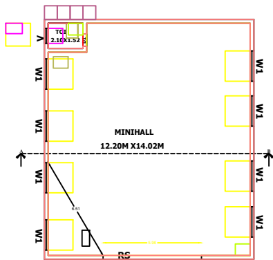
TYPICAL_FLOOR_PLAN=1
