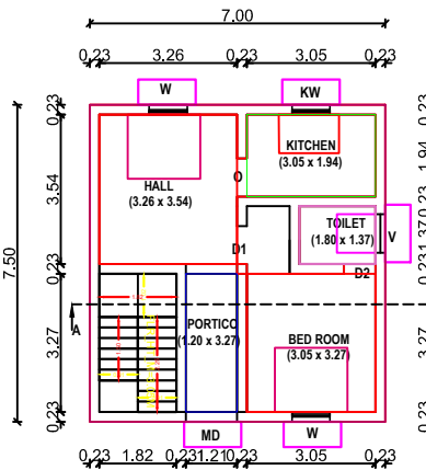
PROPOSED GROUND FLOOR PLAN
