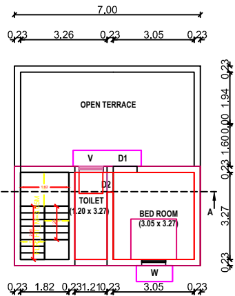
PROPOSED FIRST FLOOR PLAN
