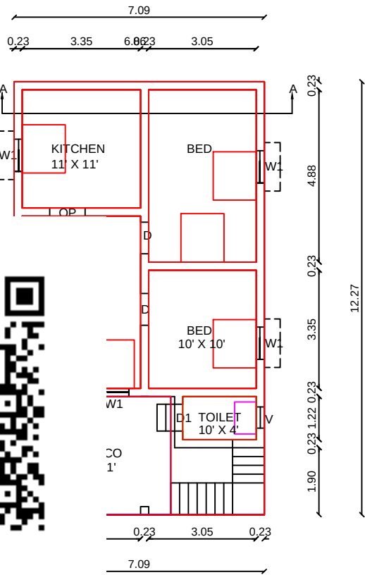
PLAN
