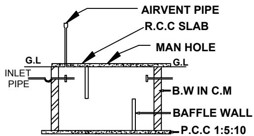
SECTION ON SEPTIC TANK
