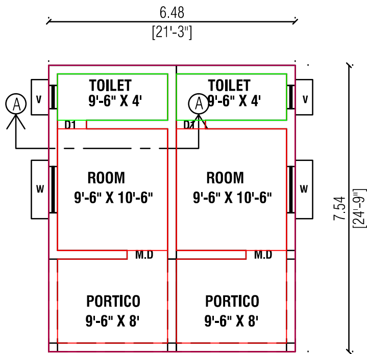
HOUSE-1 HOUSE-2 GROUND FLOOR PLAN
