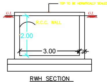
RWH SECTION
