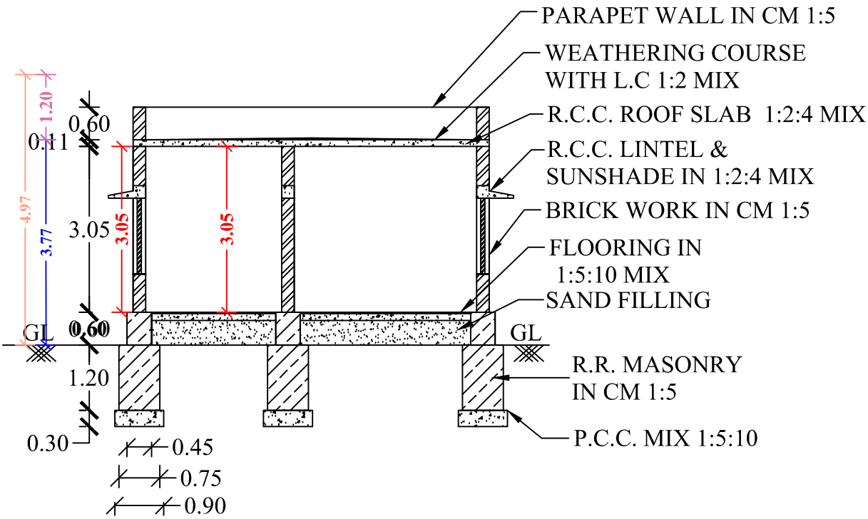
SECTION OF "AB"
