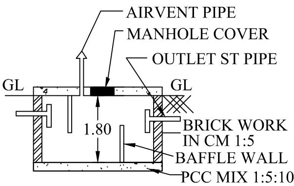
SECTION ON SEPTICTANK
