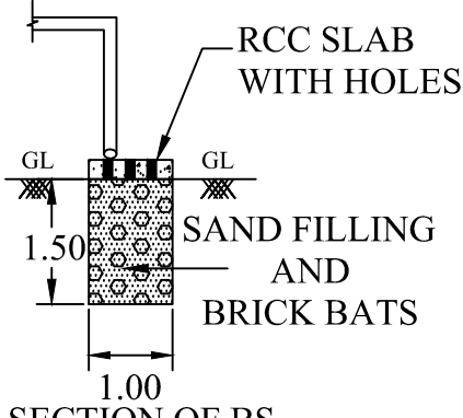
SECTION OF BS
