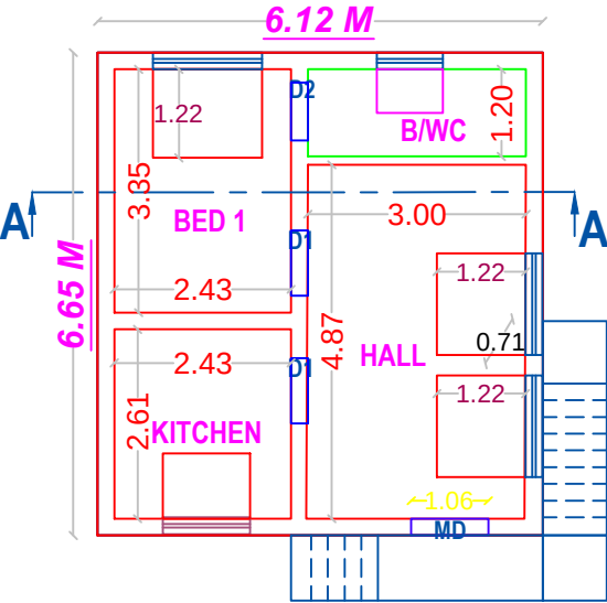
PLAN - GROUND FLOOR ( PROPOSED )
