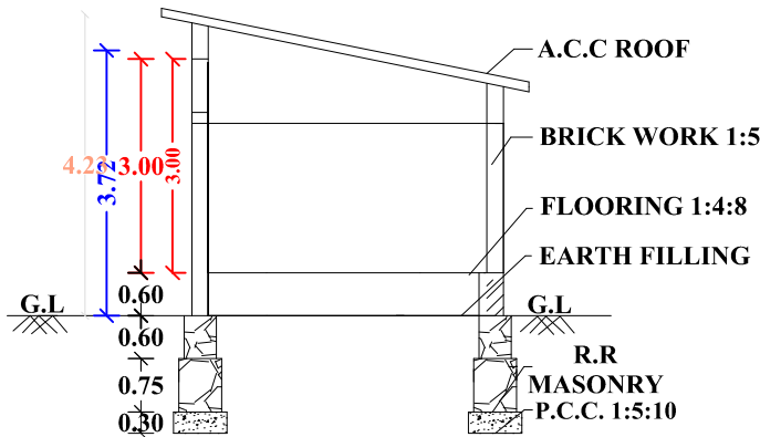
"SECTION "AB"
