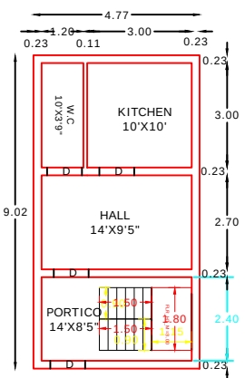
EXT GROUND FLOOR RESIDENTIAL PLAN
