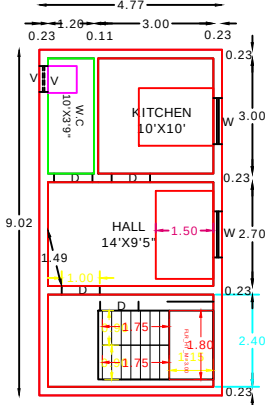
PRO FIRST FLOOR RESIDENTIAL PLAN
