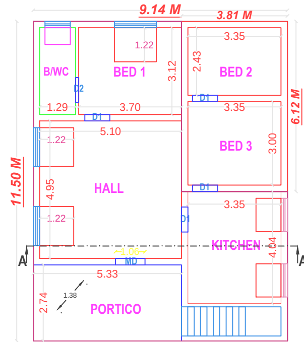
PLAN - GROUND FLOOR (ADD. PROPOSED)
