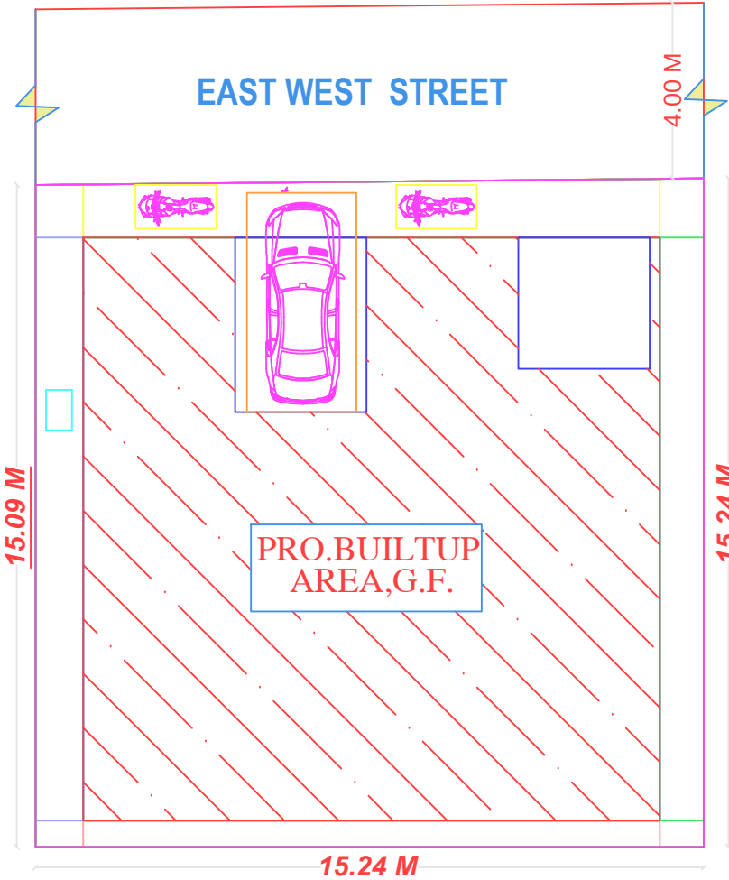
PLOT NO : 34, SANKAR MARIAPPAN LAND
