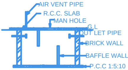
SECTION ON SEP.TANK
