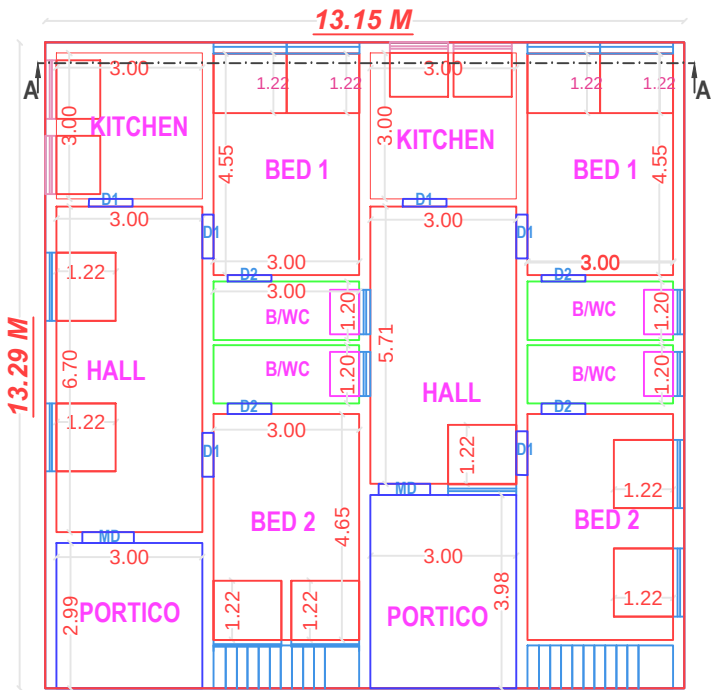
PLAN - GROUND FLOOR (PROPOSED)
