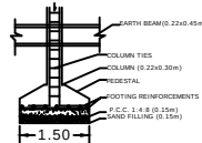
FOUNDATION DETAILS
