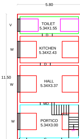
PROPOSED GF PLAN
