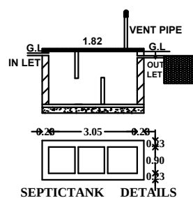
SEPTICTANK DETAILS
