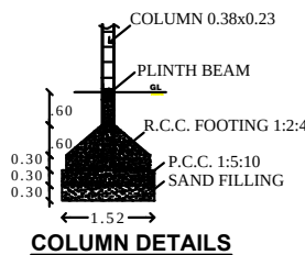
COLUMN DETAILS
