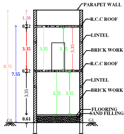
"SECTION "AB"
