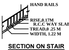
SECTION ON STAIR
