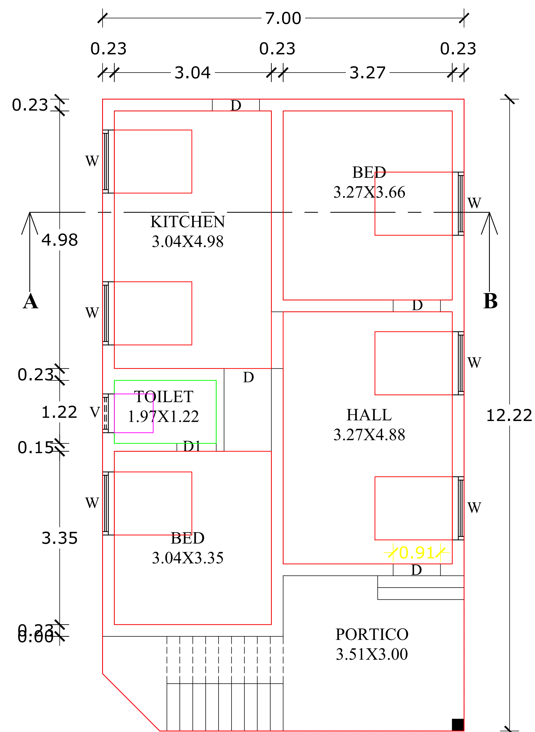
PLAN
