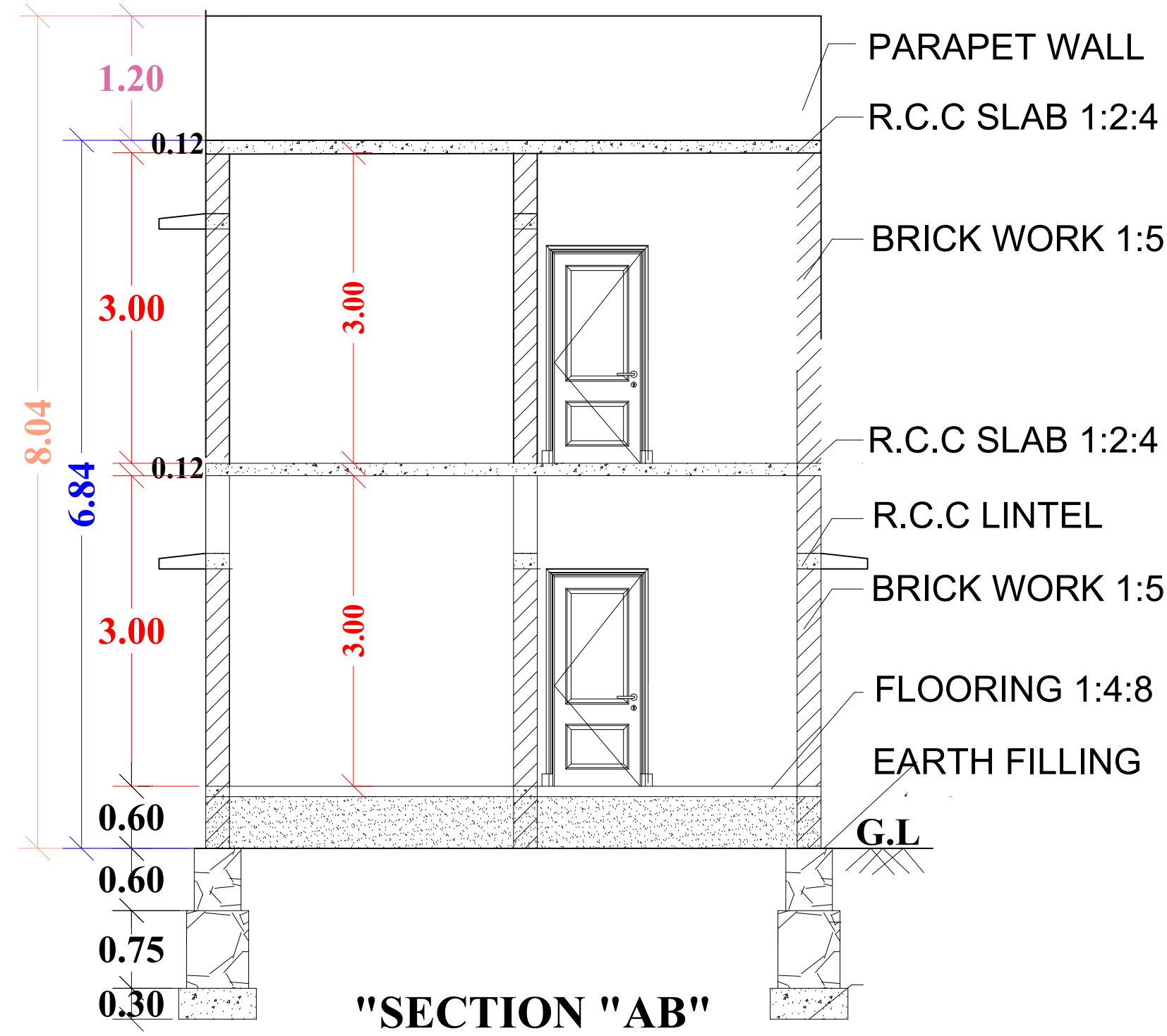
"SECTION "AB"
