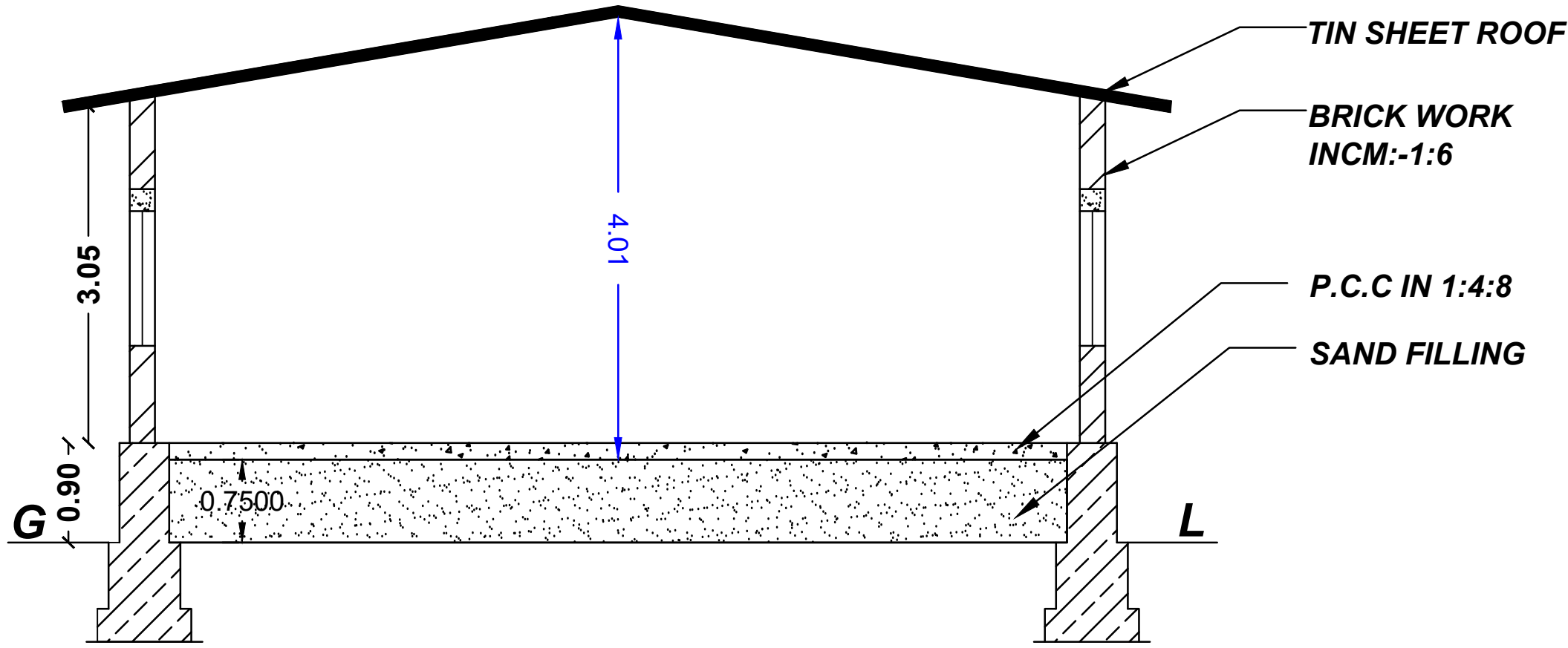
SECTION "AB"
