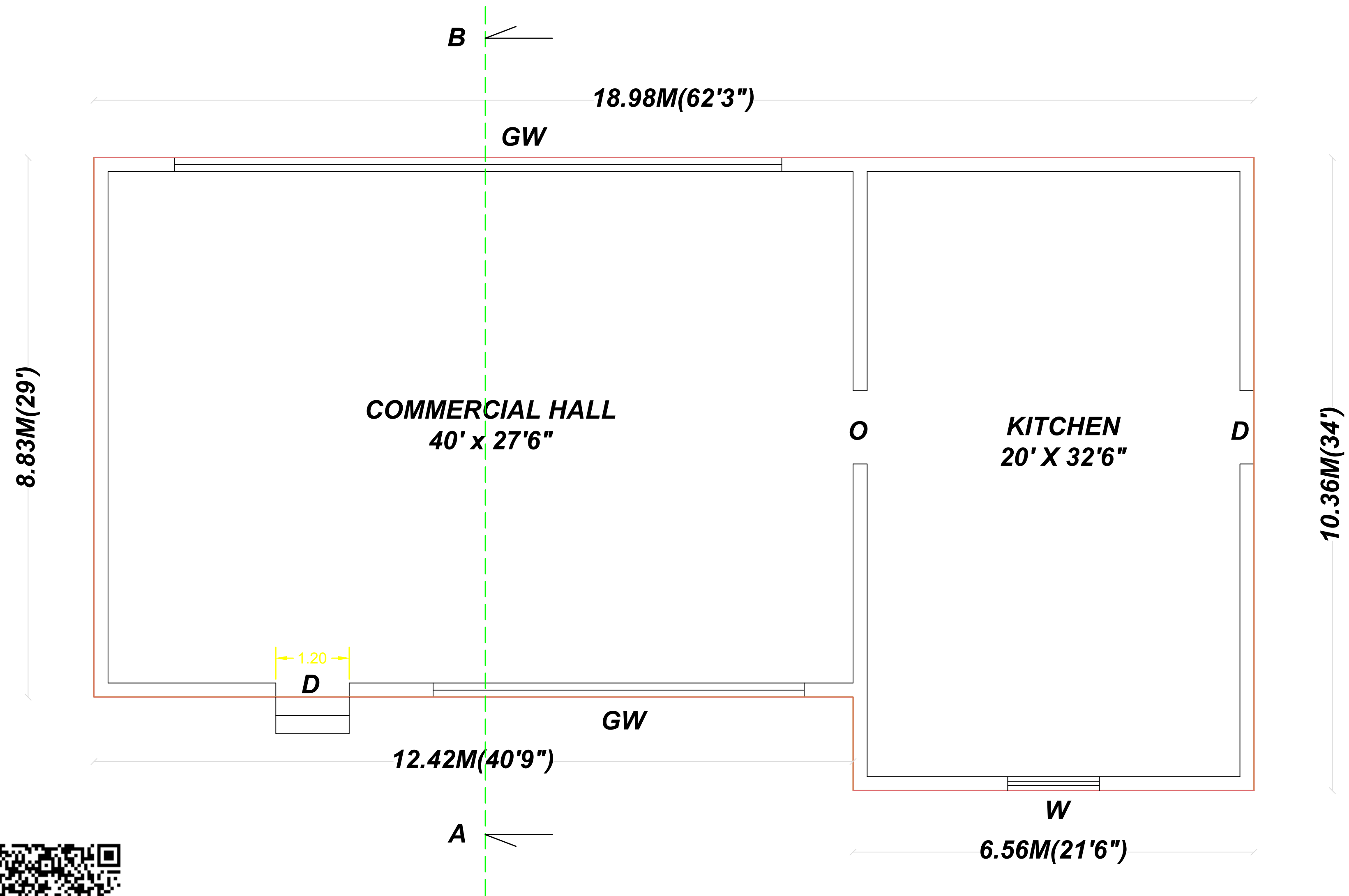
PLAN
