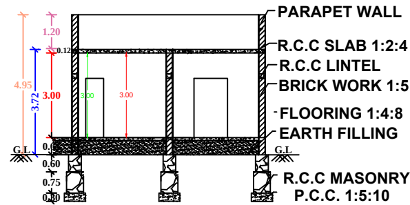
"SECTION "AB"
