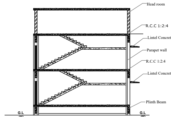
SECTION ON-AB
