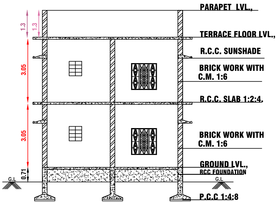
SECTION ON A-A & A'-A'
