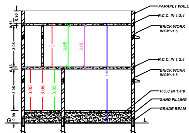
SECTION "AB"
