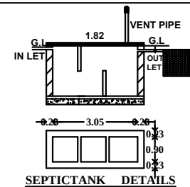
SEPTICTANK DETAILS
