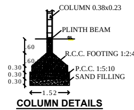
COLUMN DETAILS
