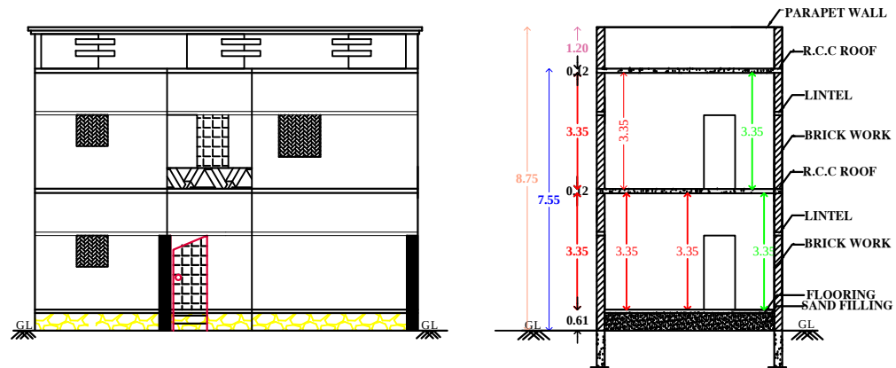
"SECTION "AB"
