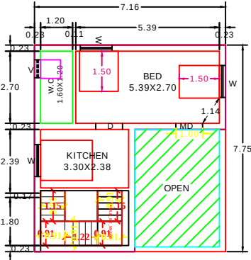
PRO FIRST FLOOR RESIDENTIAL PLAN
