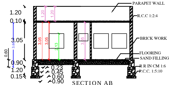
SECTION AB
