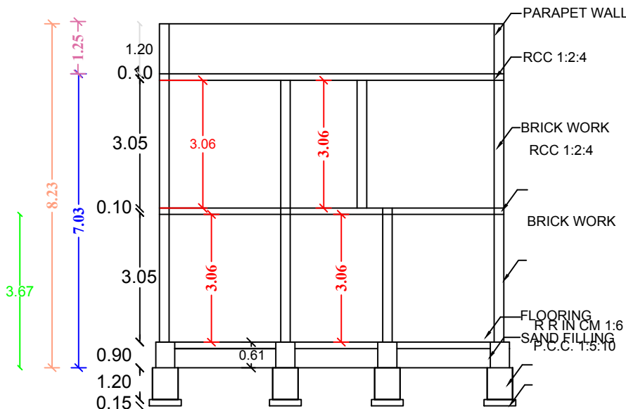
SECTION AB
