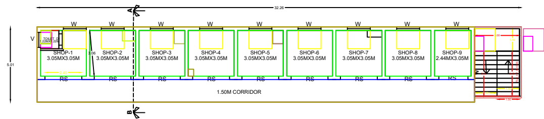
PRO.FIRST FLOOR PLAN
