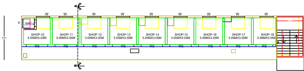
PRO.FIRST FLOOR PLAN
