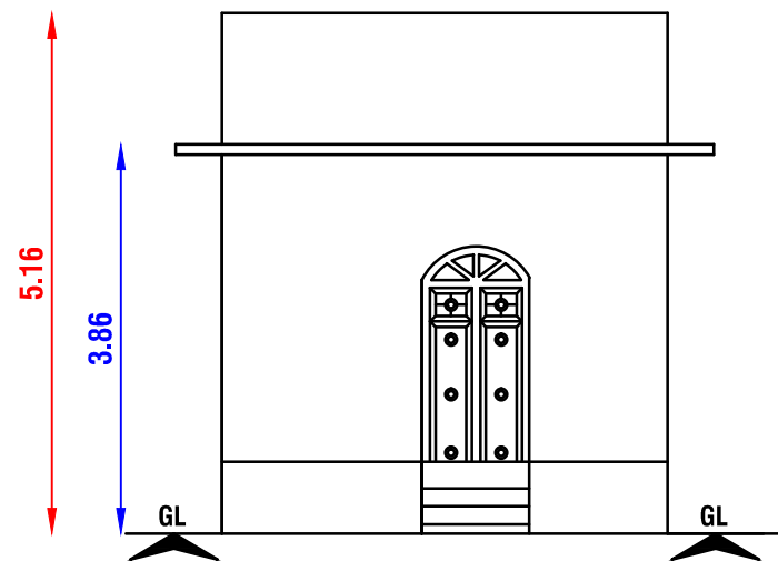
FRONT ELEVATION
