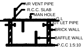
SECTION ON SEPT.TANK
