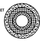
PLAN LEACH WELL DETAIL
