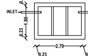
PLAN SEPTIC TANK DETAILS
