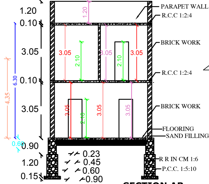
SECTION AB
