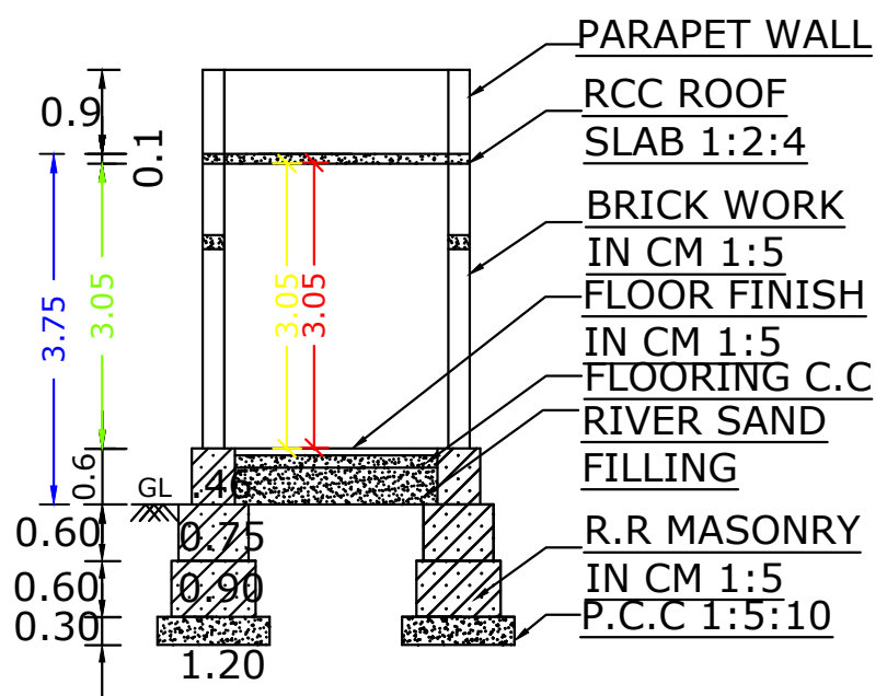
SECTION ON AA1
