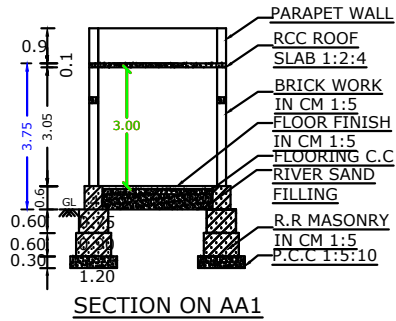
SECTION ON AA1
