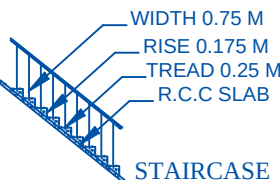
STAIRCASE
