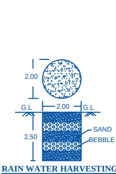
RAIN WATER HARVESTING
