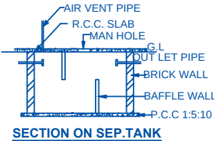
SECTION ON SEP.TANK
