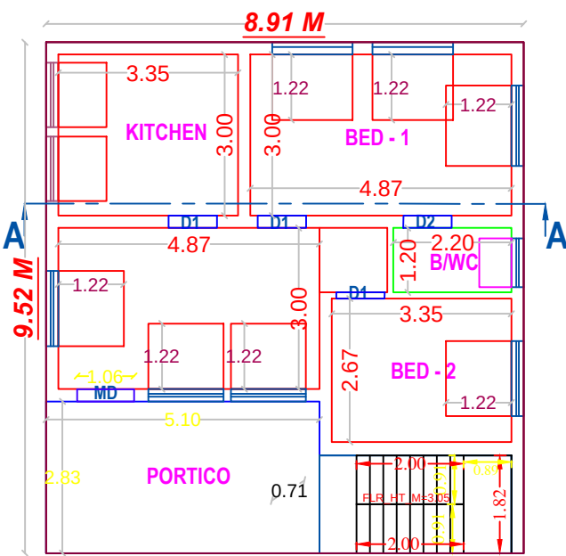
PLAN - GROUND FLOOR ( PROPOSED )
