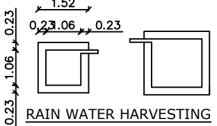
PERCOLATION PIT
