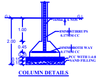
COLUMN DETAILS
