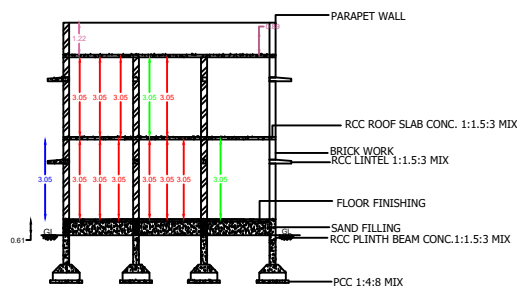
SECTION AB
