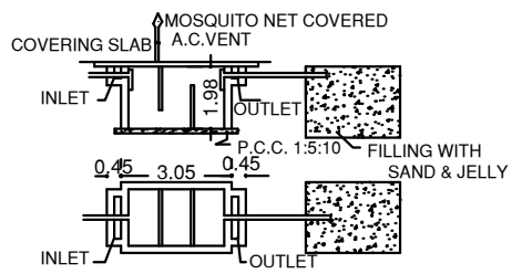
SEPTIC TANK & TRENCH U TRAP PROVISION
