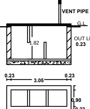
SEPTIC TANK
