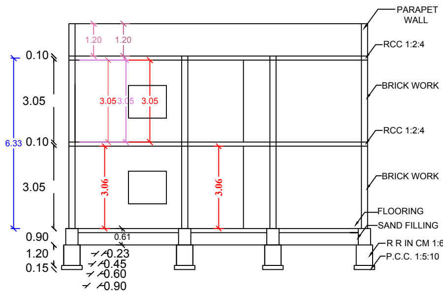
SECTION AB
