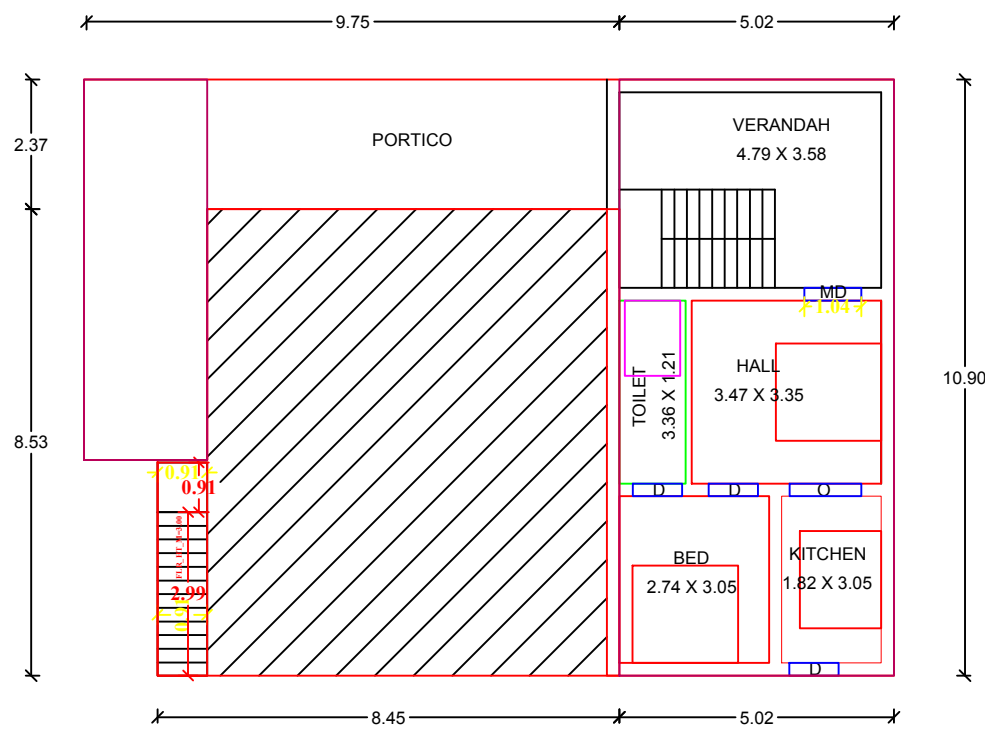
FLOOR PLAN
