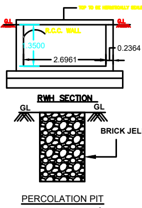
PERCOLATION PIT
