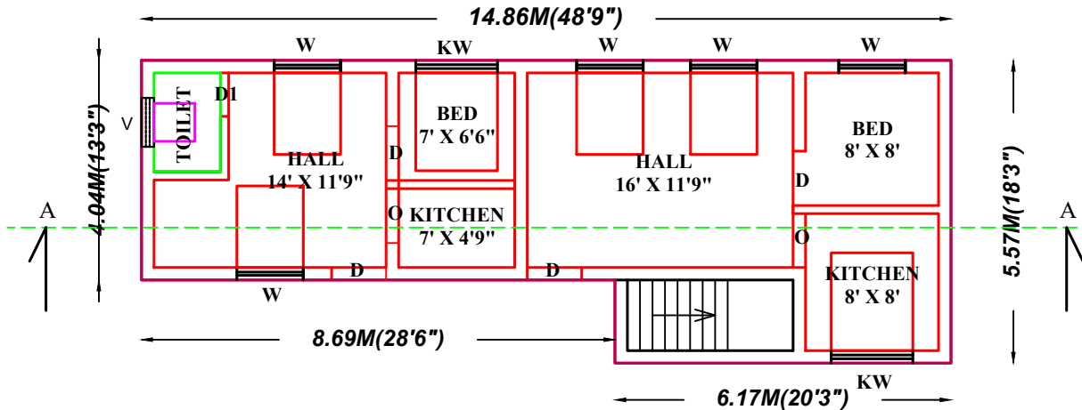
PLAN
