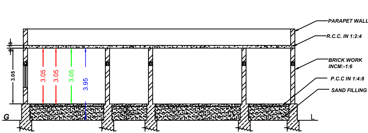
SECTION "AB"
