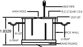
SECTION E.E. SEPTIC TANK DETAIL
