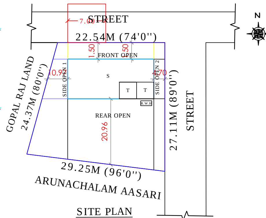
SCALE 1:200
